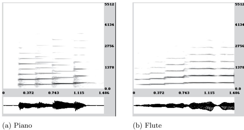
Fig. 3.3 Two spectrograms.
